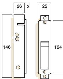
SP3540 -LS Latch Strike Fabricator Mounting
