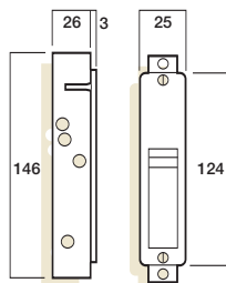
SP3540-SS Security Strike Fabricator Mounting
