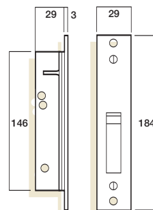
SP3640-SS Latching Strike Timber/Metal Jamb
